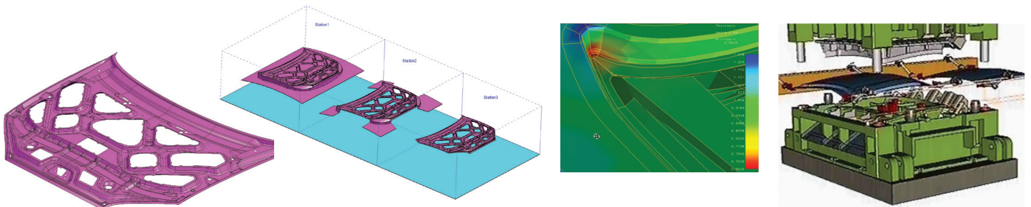
Part design
