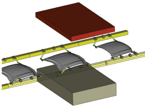
Transfer motion analysis
