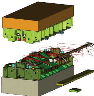
Collision check during Simulation
