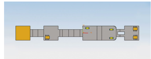
Flexible PCB design enables users to flatten a PCB for manufacturing or other purposes.
