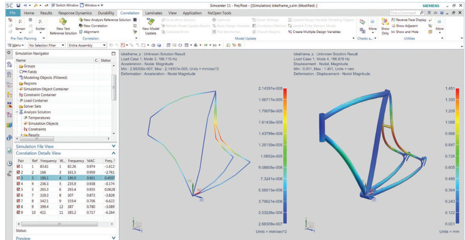
Mode pairs and side-by-side animation test/analysis.
