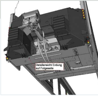
Coupling assembly after crash box – a Process Simulate analysis.
